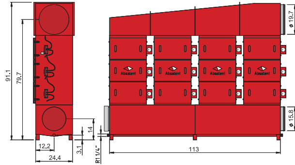
ODF 8000 with outlet side, fan not included
