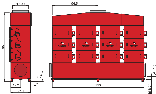
ODF 8000 with centred outlet, fan not included
